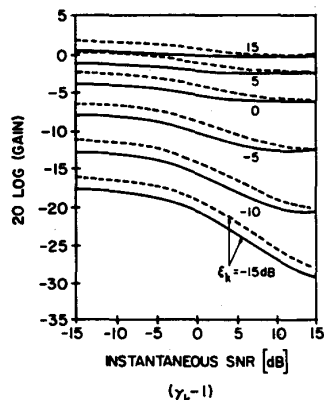
Fig. 1. Parametric gain curves. Solid line: STSA(20). Dashed line: MMSE-STSA ([1], formula (7)).
