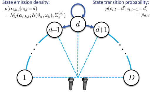
Fig. 1. The time-varying frequency array response for each source is modeled by an HMM. The DOA indices d = 1, \dots, D correspond to the hidden states and the time sequence of frequency array responses \mathbf{a}_{i,k,1}, \dots, \mathbf{a}_{i,k,L} corresponds to the output sequence of the HMM, respectively.
